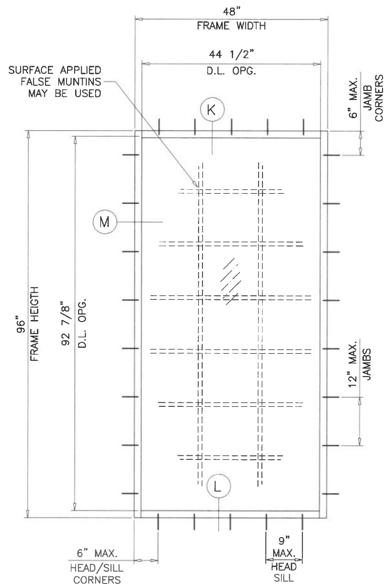
TYPICAL ELEVATION ( O )
