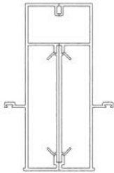
DOOR TO FIXED PANEL MULLION
